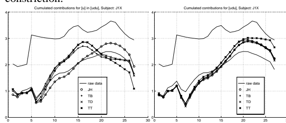
Figure4: [u] and [d] in an [udu] sequence by J1X
