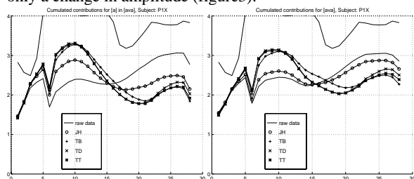
Figure3: [a] and [v] in an [ava] sequence by speaker P1X
