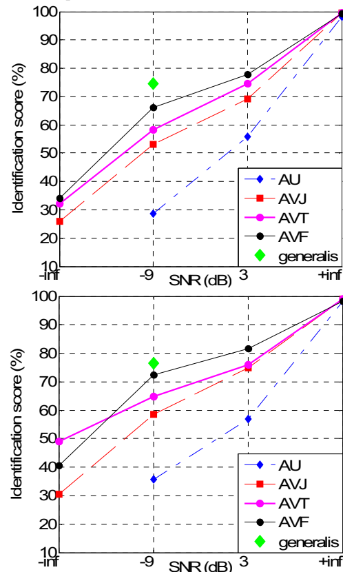
Figure 2 – Mean identification scores as a function of SNR (top: group I; bottom, group II) for the different conditions (from bottom to top): AU, AVJ, AVT, AVF. The isolated diamond indicates the score for the generalisation test.
