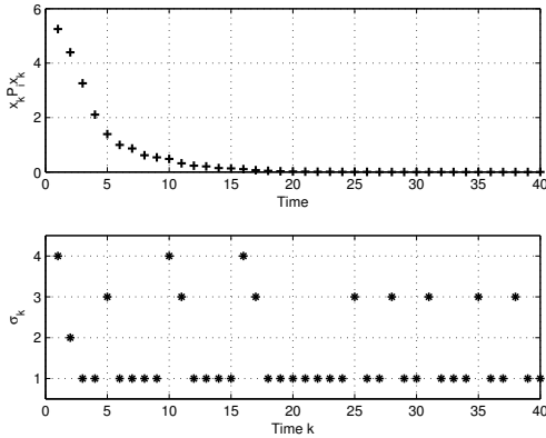
Fig. 3. Lyapunov function and switching control law in time.
