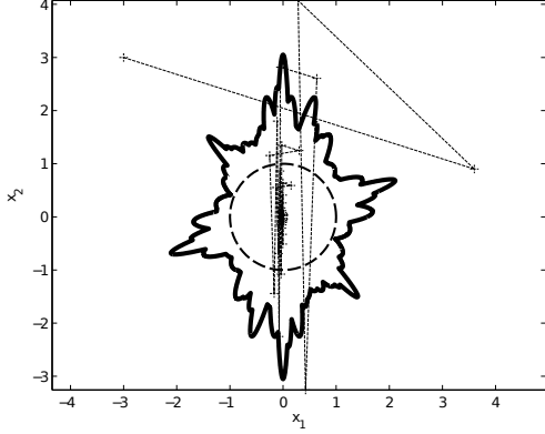
Fig. 2. Ball \mathbb{B}^2 in dashed and \bigcup_{k \in \mathbb{N}_5} \Omega_k in solid line. Trajectory starting from x_0 = (-3, 3)^T in dotted line.
