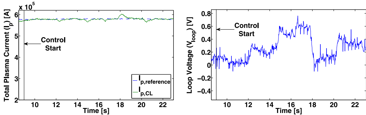
(a) Tracking of the total plasma current.
