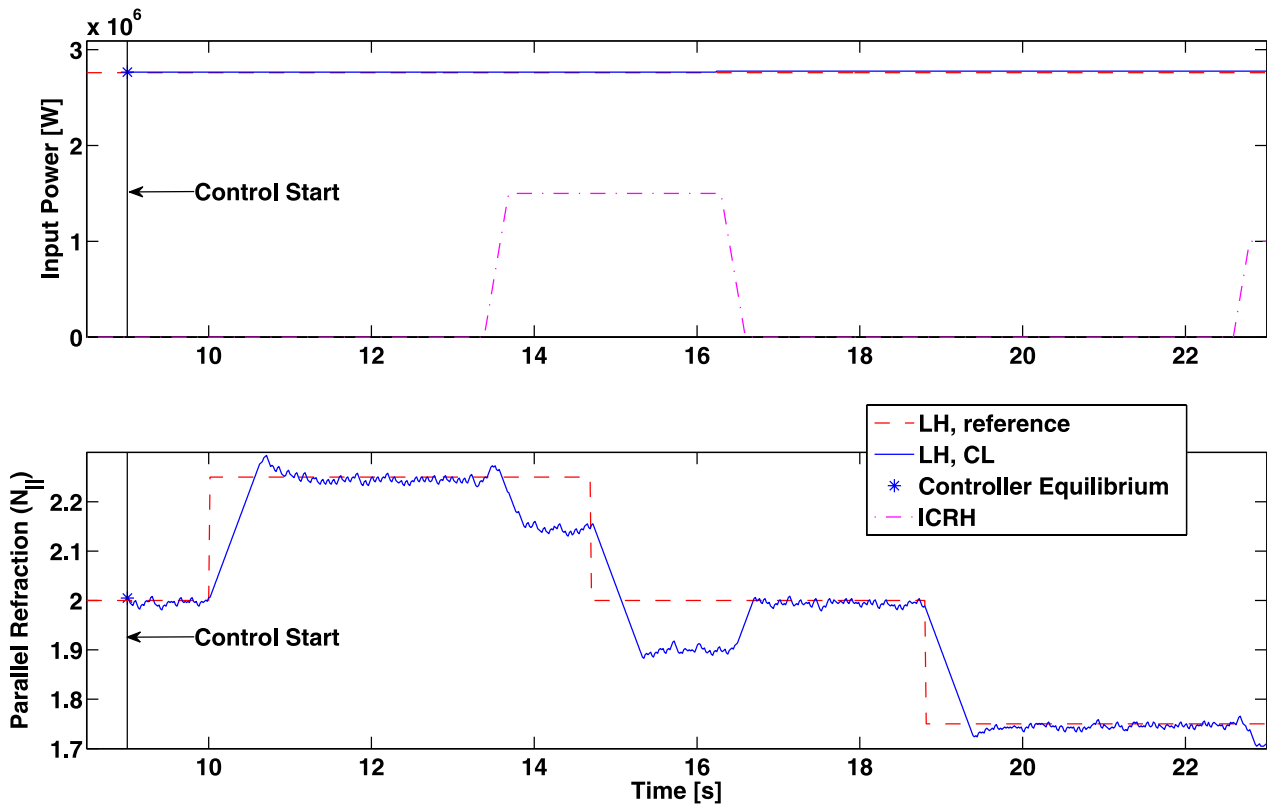
(b) Controller action and ICRH disturbance.
