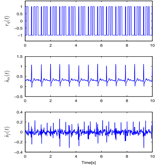
Fig. 3: Extraction of fetal ECG using a 1-bit reference with Gaussian process: r(t) is the thoracic reference, \hat{s}_m(t) is the maternal estimation, and \hat{s}_f(t) is the fetal estimation.
