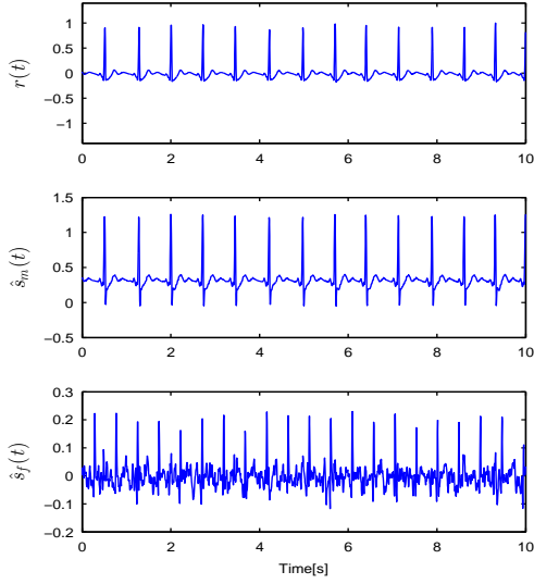
Fig. 2: Extraction of fetal ECG using a 16-bit reference with Gaussian process: r(t) is the thoracic reference, \hat{s}_m(t) is the maternal estimation, and \hat{s}_f(t) is the fetal estimation.
